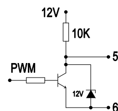
Speed setting via Bus
